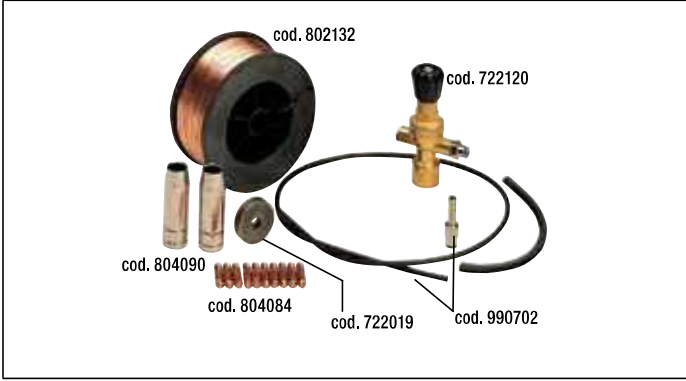
cod. 802147 - Ø 0,6mm x Bimax 140, 162, Technomig Dual Synergic, Maxima 160, 190, 200 Synergic
